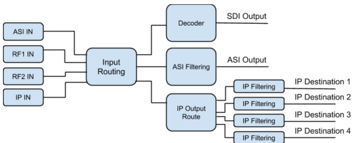
Input to Output Routing and Filtering
